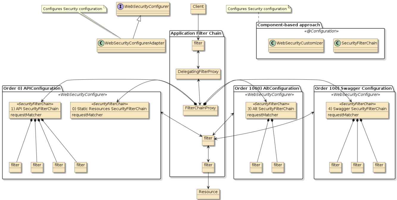
Figure 1. Multiple SecurityFilterChains
